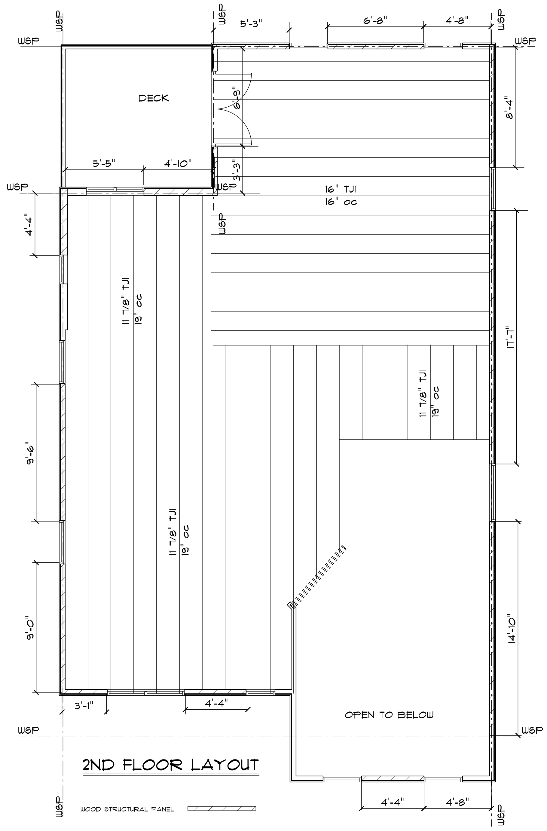
WALL PANELS & FRAMING LAYOUTS
