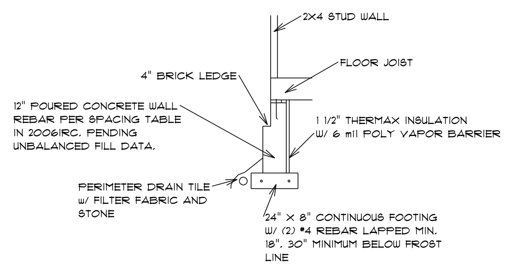
FOUNDATION DETAIL
