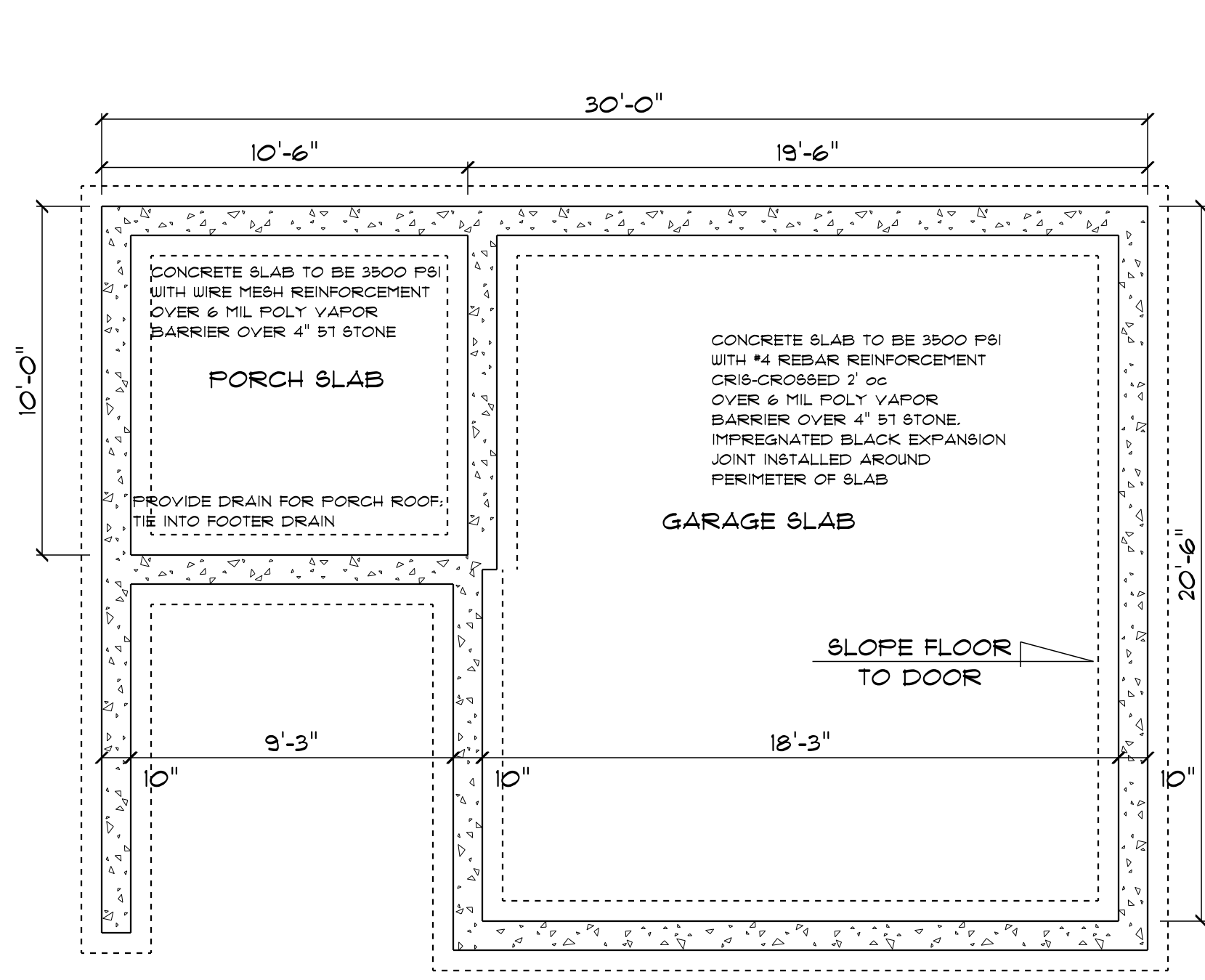
SCREENED PORCH SLAB - ALTERNATE FOUNDATION
